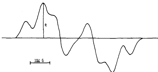
Figure 2. Determination of the EPR signal peak height at maximum amplitude in the \Delta m_s = \pm 1 spectrum of 4 in a rigid propylene glycol glass at 143.6 K.
